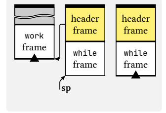
(c) Stack layout before/after resume, with the LEXA compiler. A triangle marks the boundary from a SysV function to a preserve_none function.
