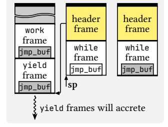
(b) Stack layout before/after resume, with setjmp and longjmp. A gray jmp_buf is populated.
