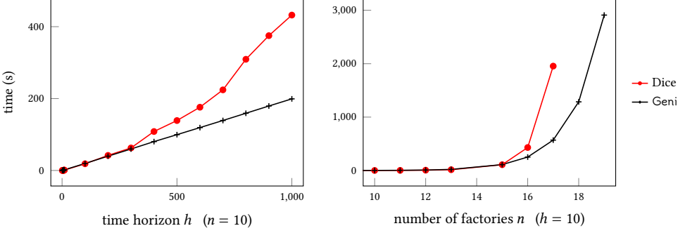
Figure 9. Scaling of Dice and Geni on a model-checking benchmark from Holtzen et al. [18]. In the right diagram, Dice times out for n \geq 18 .
