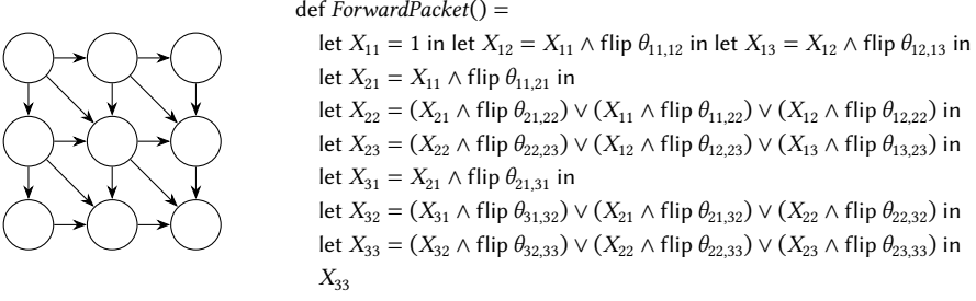
Figure 10. A 3 \times 3 grid-network model with probabilistic link failures. The model is from Fierens et al. [13]. Left: network topology. Right: Geni function modeling the probabilistic behavior of the network.
