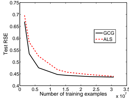
Figure 3: Test RSE on Yelp
