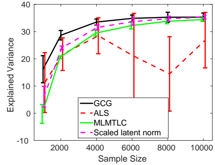
Figure 6: School grade prediction
