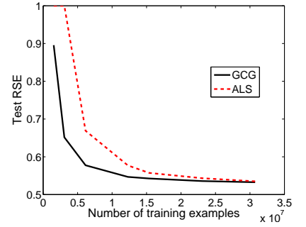
Figure 4: Test RSE on Nell
