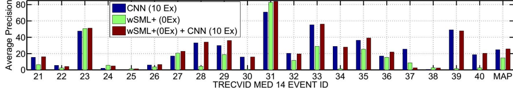
Figure 4: Performance comparison of CNN on MEDTest 2014 dataset, wSML+, and the hybrid of CNN and wSML+.
