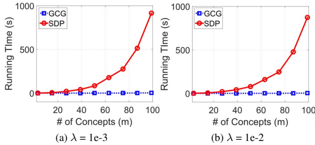
Figure 2: Efficiency comparison between GCG and SDP.
