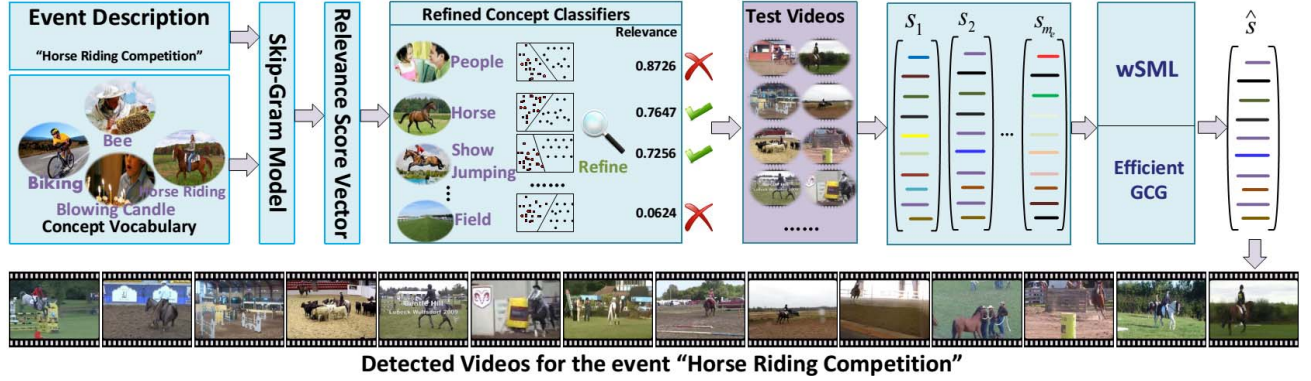
Figure 1: The proposed framework for large-scale semantic event search (§3), illustrated on the particular horse riding competition event. The relevance of concept classifiers to the event of interest are measured using the skip-gram language model (§3.2), followed by some further refinements (§3.3). To account for their reliability, the concept scores are combined through the warped spectral meta-learner (§3.6) and solved using the efficient GCG algorithm (§3.7).
