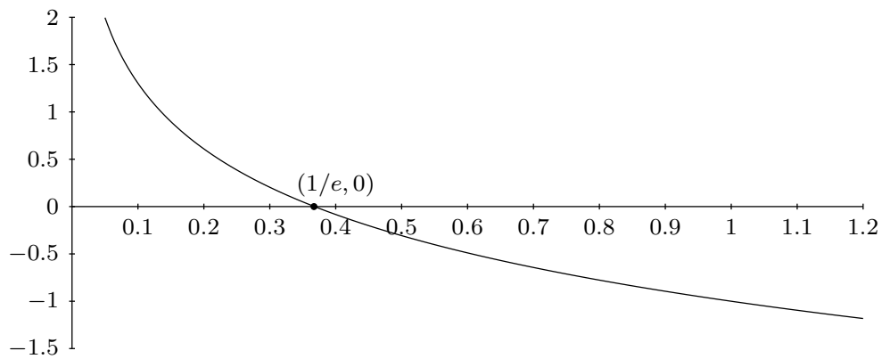
(b) \eta'(\alpha) = -(1 + \ln(\alpha))
