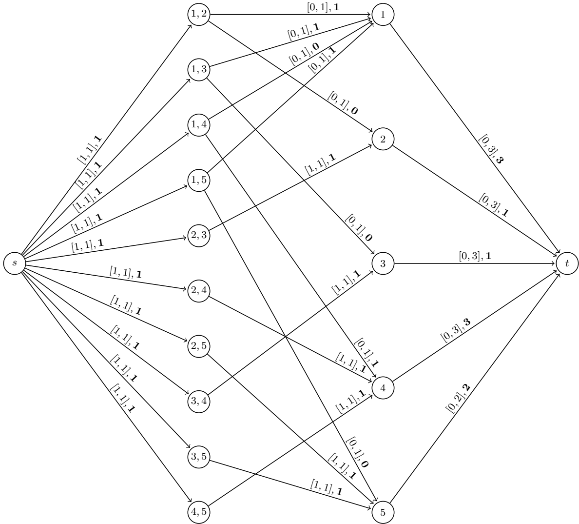
Figure 4.4: The feasible flow network from Example 4.6. The edges are denoted with upper and lower bound capacities in the brackets and a corresponding feasible flow, shown in bold. The conspirator (Team 1) can change each of the games they were supposed to win but all other games are fixed.
