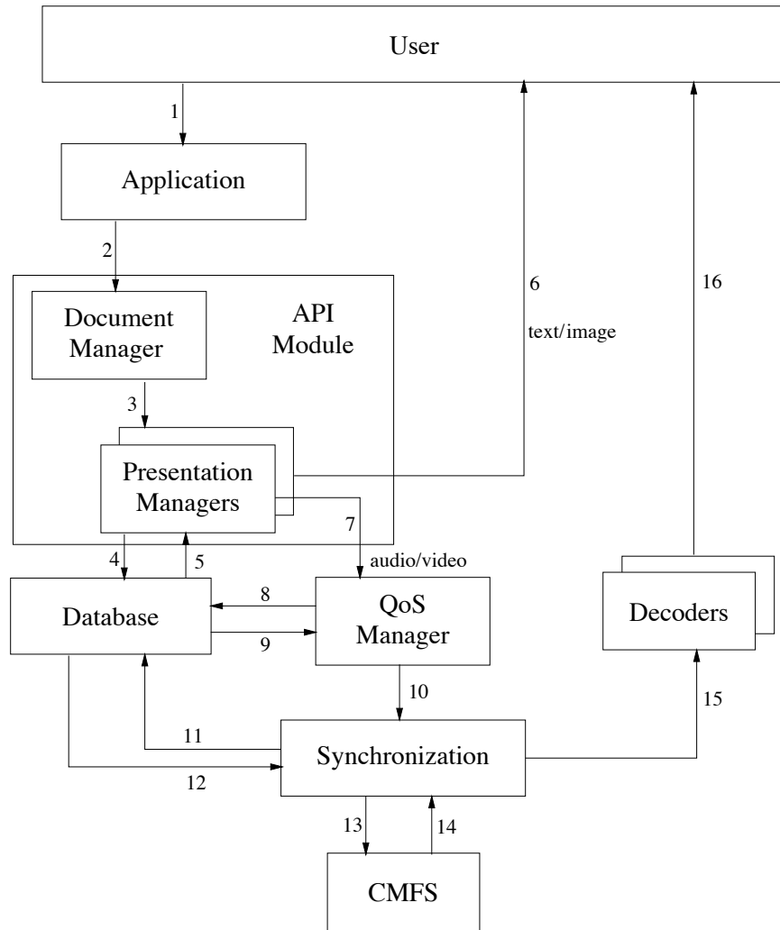
Figure 4: Steps required to display a document
