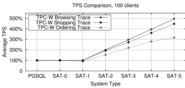
Fig. 6 Ganymed Performance for TPC-W Mixes.
