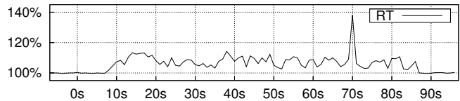
Fig. 16 Effect of Replication on Source Machine
