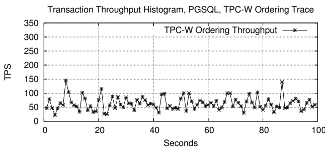
Fig. 7 Example Histograms for the TPC-W Ordering Mix.
