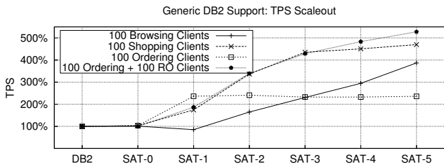
Fig. 12 Measurement Results for DB2 with the Generic Approach.
