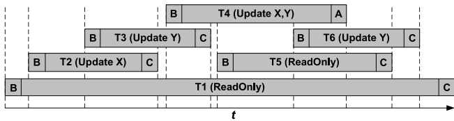
Fig. 5 An example of concurrent transactions running under SI.
