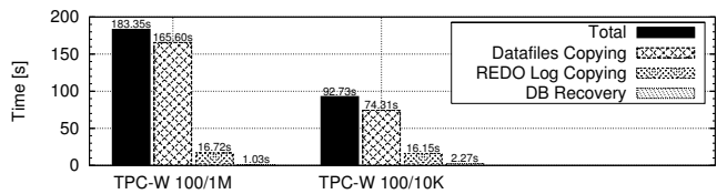
Fig. 15 Replication Times with PITR
