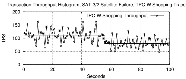
Fig. 8 Ganymed reacting to a Satellite Failure.
