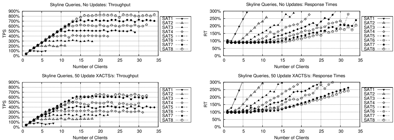
Fig. 13 Skyline Performance Results
