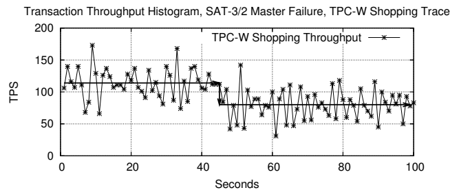
Fig. 9 Ganymed reacting to a Master Failure.
