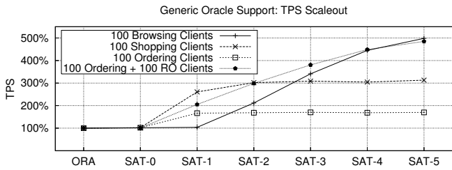
Fig. 11 Measurement Results for Oracle with the Generic Approach.
