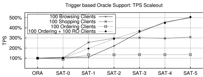
Fig. 10 Measurement Results for Oracle with the Trigger based Approach.
