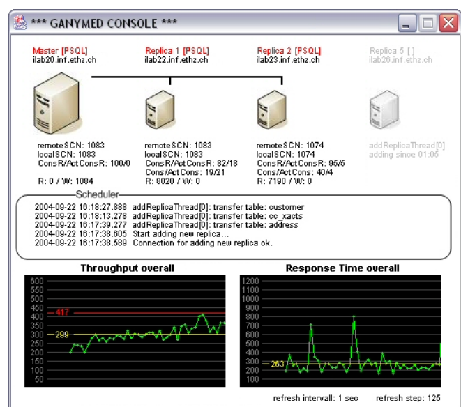
Fig. 4 The Management Console.
