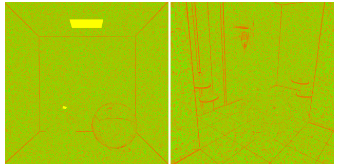
Figure 6: The ratio of the estimated bias and the estimated noise bound in error estimation with 15M emitted photons. The red pixel indicates the bias is dominant and the green pixel indicates the noise is dominant in the estimated error. The result for the flashlights scene is in Figure 1.
