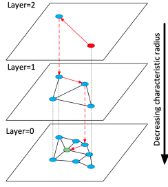
Figure 1: HNSW Index (replicated from reference [22]).
