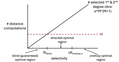
Figure 4: Optimal selectivity regions of fixed heuristics.
