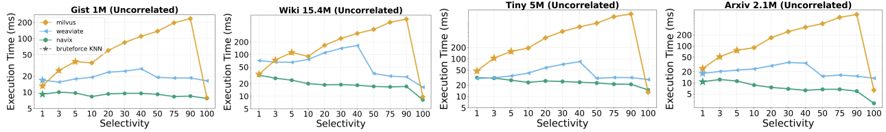
Figure 12: Execution Time vs Selectivity for prefiltering baselines at 95% recall
