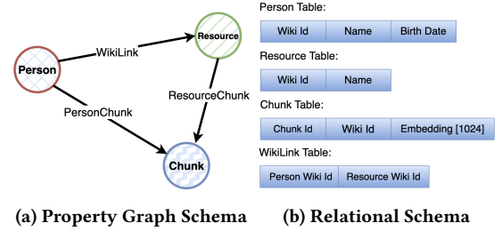
Figure 7: Wiki Schema
