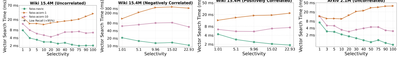
Figure 13: Vector Search Time vs Selectivity for ACORN and Faiss-Navix baselines at 95% recall
