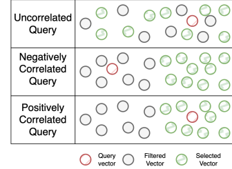
Figure 5: Pictorial depiction of different correlations S can have with v_Q 's neighborhood. Replicated from reference [32].
