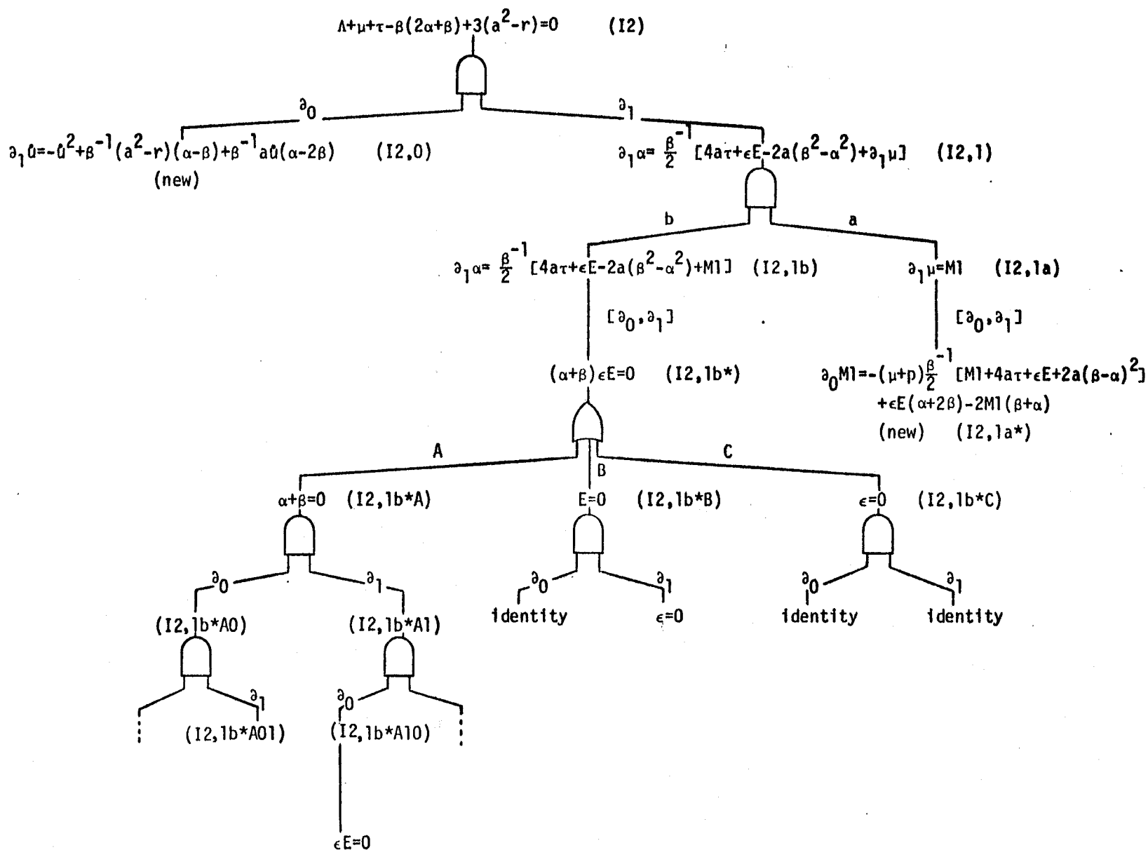
Figure 4.3.1: I2: 123 = 0 and \beta \neq 0
