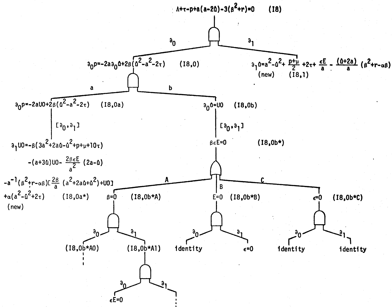
Figure 5.2.4: I8: 023 = 0 with a \neq 0
