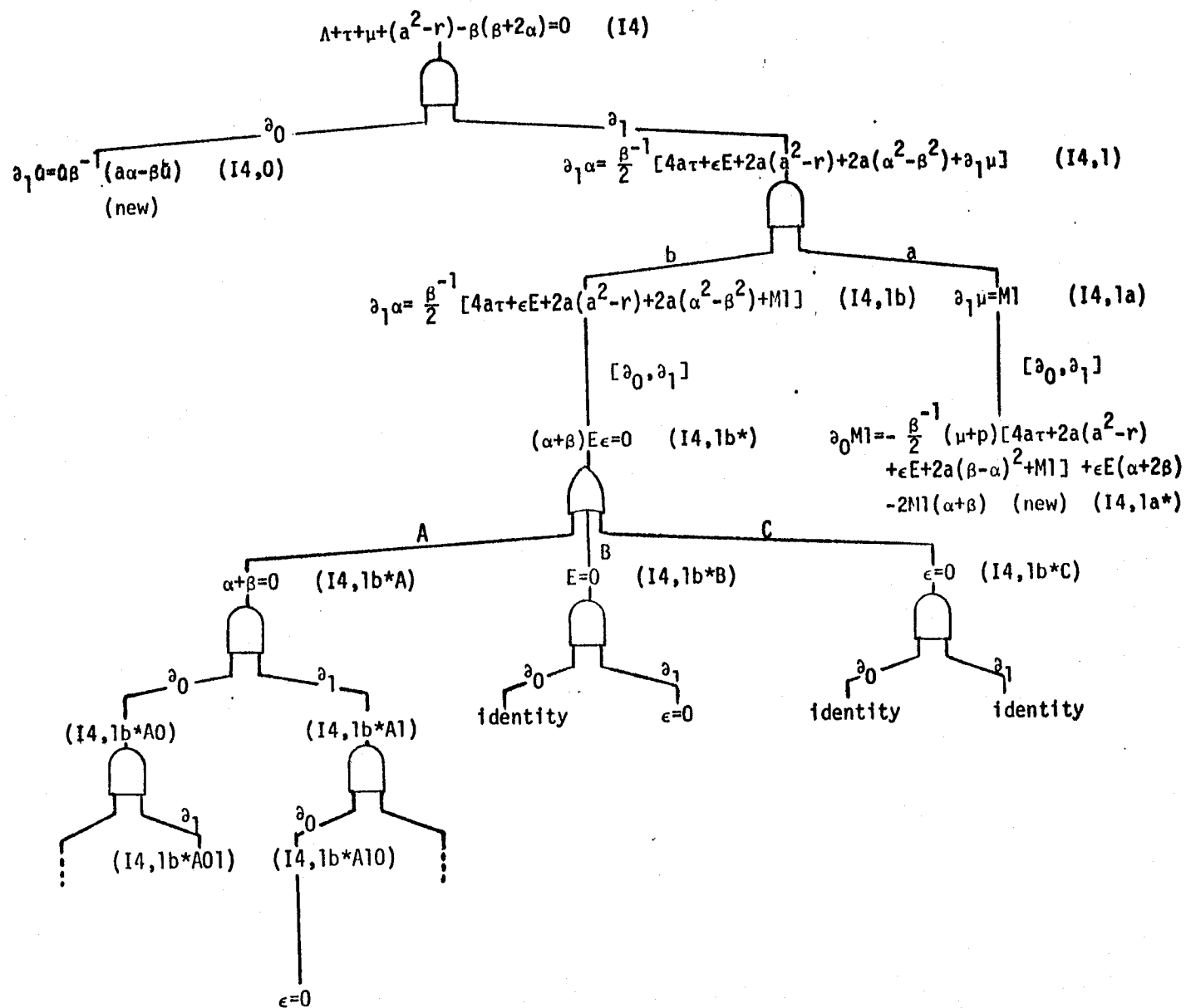
Figure 4.4.1: I4: \frac{1}{2}R = 0 and \beta \neq 0
