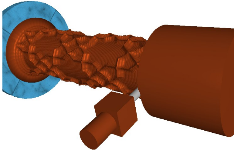
Fig. 6. A picture from the milling lathe simulator. The simulator is shown cutting the cylindrical star pattern pictured in Figure 4(b).
