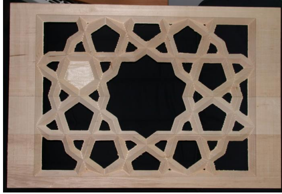
Fig. 2. A sample star pattern cut with a traditional 3-axis NC milling machine using the technique discussed in Section 2.1.
