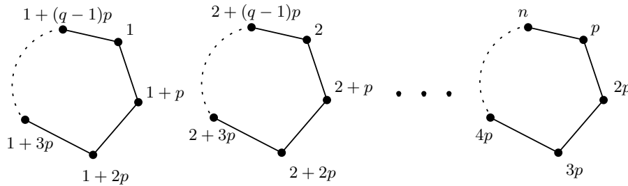
Figure 3.11: The graph G .
