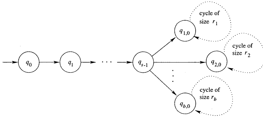
Figure 1: Constructing an NFA
