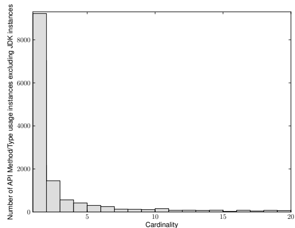
Figure 4: A histogram of the cardinality values obtained when the tool was run on the 4,000 code snippets described in Table 5.1.
