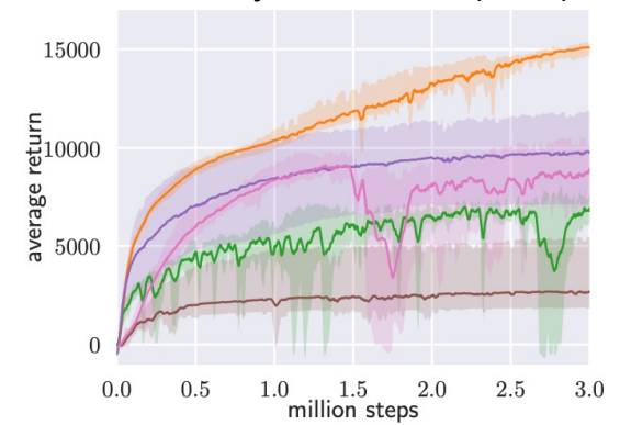
(c) HalfCheetah-v1
