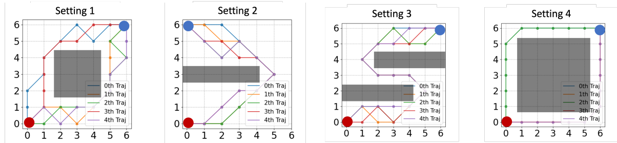
Figure 7: The Grid-World Environments: We randomly select five expert trajectories (denoted as 0 th Traj to 4 th Traj) for visualization purposes. The starting point and destination are denoted by red and blue circles, respectively. The primary objective of the ICRL algorithms is to deduce the constrained region, which is unobservable and illustrated by the gray color.
