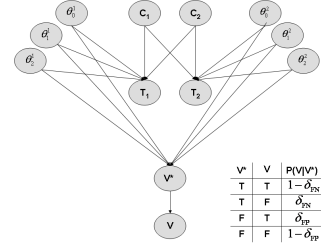
Figure 3: Augmented network extended to handle inaccurate feedback
