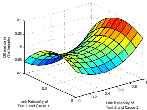
Figure 4: Difference in Gini impurity for the network in Fig. 1 when \theta_2^1 and \theta_2^2 are the only parameters allowed to vary.
