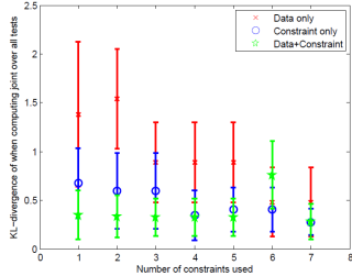
Figure 7: Mean KL-divergence and one standard deviation for a 3 cause 3 test network on learning with data, constraints and data+constraints.
