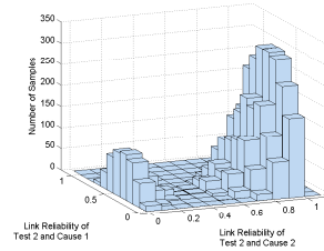
Figure 6: Posterior over parameters calculated through Sampling.
