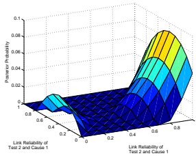
Figure 5: Posterior over parameters computed through calculation after discretization.
