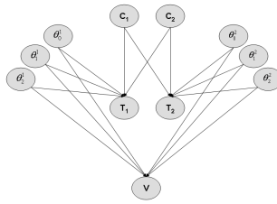
Figure 2: Augmented network with parameters and constraints
