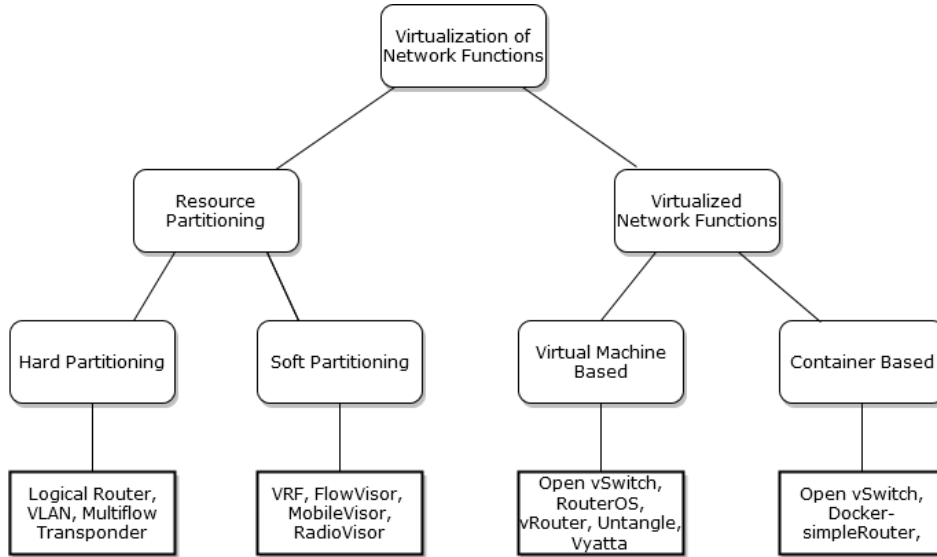
Figure 1.1: Technologies for virtualizing network functions with examples
