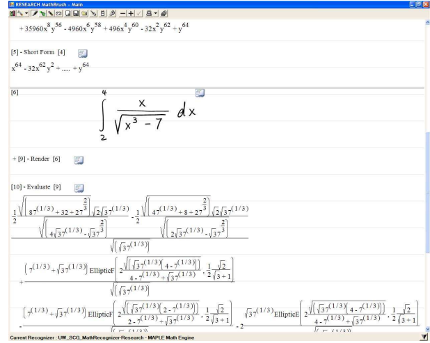
Figure 1: MathBrush User Interface, showing both input and the rendering of a long output string. The output display heuristics try to keep fractions, parentheses, etc. together, and prohibit horizontal scrolling. For example, for fractions, as line-breaking becomes necessary, the system may transform rendering of a fraction from \frac{\text{numerator}}{\text{denominator}} to \frac{1}{\text{denominator}} * (\text{brokenNumerator}) , or to (\text{brokenNumerator})/(\text{brokenDenominator}) depending on the length of numerator and/or denominator.
