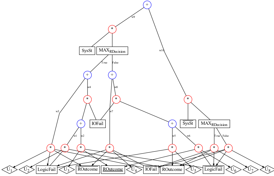
Figure 3: An example SPMN learned from the Computer Diagnostician dataset using LearnSPMN. The partial order used is \{SysSt\} \prec RDecision \prec \{LogicFail, IOFail, ROutcome\} .
