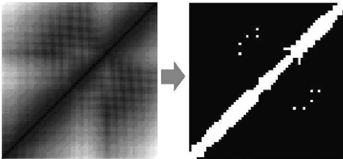
Figure 2.11: The image on the left is a distance map derived from the PDB file for one chain of the protein with PDB ID a1o1, a transcription factor (DNA). The darker the region, the closer those two amino acids are in space. The diagonal axis is black, as an amino acid is distance 0 from itself. The distance map has been converted to the contact map on the right by applying a threshold of 7Å to the distance map. In the contact map a white square indicates a true value, meaning that those amino acids are within the threshold distance of each other. Notice the smattering of white squares distant from the central axis in the contact map. These represent contact between regions of the protein which are distant from each other on the backbone. These are the regions where we will find the contacts for supersecondary structures.
