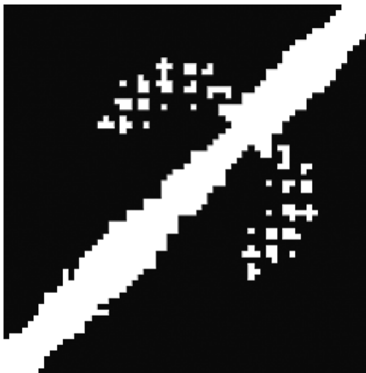
Figure 2.12: This is a contact map for the same protein (1a1o1) that was used for Figure 2.11 on page 26. Notice that in this case, there is much more information corresponding to the supersecondary structures. With a threshold of 7\text{\AA} , we would often have a contact interface with only one point of contact. By increasing the threshold to 10\text{\AA} , we are increasing the amount of information available to describe the interface.
