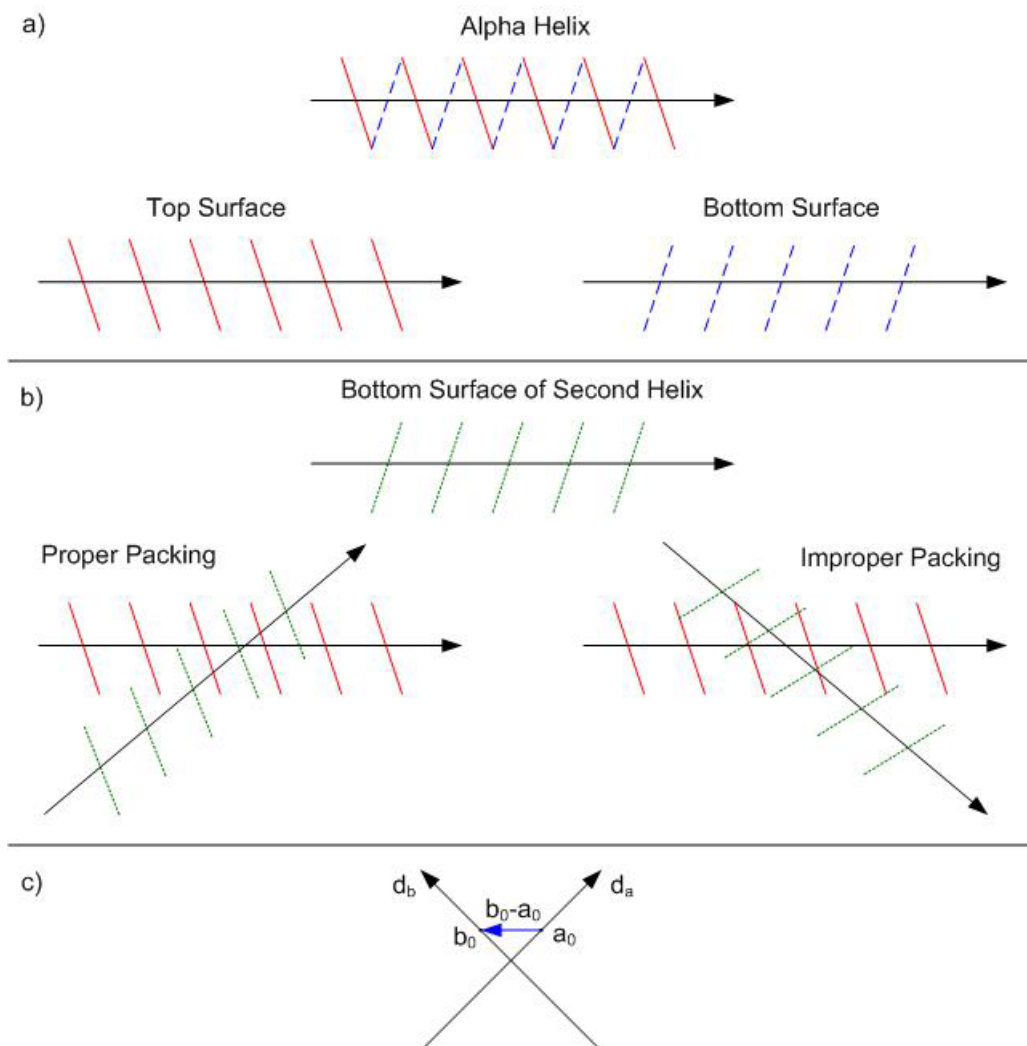
Figure 4.17: a) The top image represents a simplified alpha helix. The black arrow is the helix axis, and is lying in the plane of the page. The red lines are the sections of the helix backbone that may be considered the top surface; they are projecting out of the page. The blue lines are the bottom surface, and are beneath the surface of the page. These two surfaces are shown separately below the top image for clarification. b) The green lines represent the ridges on the bottom surface of a second alpha helix. In the two images below, this helix has been superimposed on the top surface from part a) at an angle of 45^\circ . Notice that there is a significant difference in the resultant packing, therefore a sign must be used: the left image is negative, the right is positive [CLR81] (using the right-hand rule, find the angle from the upper helix to the lower one). c) Two vectors d_a and d_b , each representing one of the helix axes, are shown.
