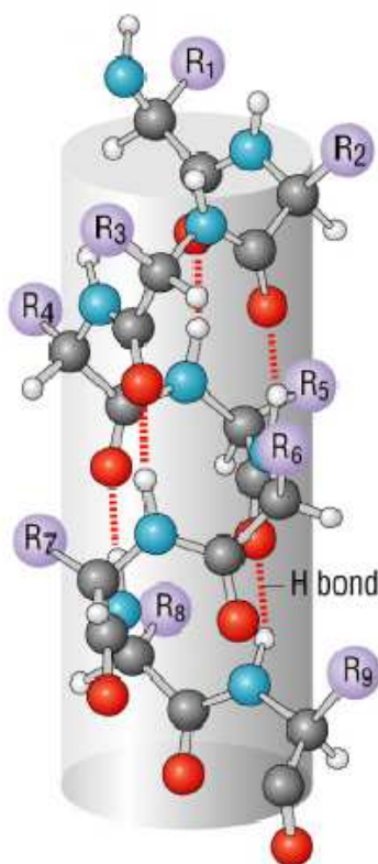
Figure 4.3: It is evident from this diagram that the side chains of an alpha helix are not perpendicular to the axis of the helix. Thus, the directionality of the helix axis is significant when considering packing. This figure has been adapted with permission from [PR04].
