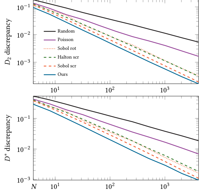
Fig. 2. L_2 and star discrepancy values ( D_2 and D^* ) for different sizes N of point set under a 2D uniform distribution. In addition to random and Poisson disk, we compare against the other analytic baselines, scrambled Halton and rotated or scrambled Sobol. Our optimization starts from scrambled Sobol points. Our method can successfully reduce both discrepancy values beyond the most common baseline of scrambled Sobol despite optimizing only a differentiable variant of the L_2 discrepancy.
