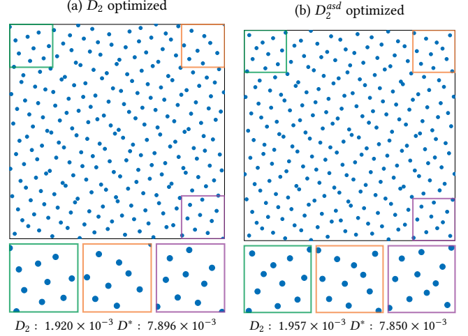
Fig. 1. Comparison of point sets optimized for uniform density by minimizing D_2 and D_2^{asd} . (a) Using origin-anchored boxes overemphasizes the origin, leading to less uniform coverage near the other corners of the domain. (b) Using all corners as anchors and averaging their D_2 discrepancies yields more uniform coverage across the entire domain.
