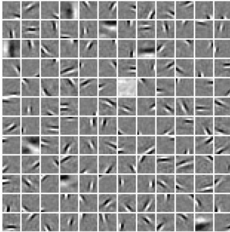
Figure 4. The set of 144 basis functions learned after training on 12 \times 12 image patches extracted from natural scenes. Details are provided in [15]. Note that these functions represent the feedforward weighting function contributing to each unit's output, and hence are not strictly equivalent to the unit's 'receptive field' because the recurrence and sparseness terms of equation (3) would also need to be taken into account. Mapping out the spatial response of each unit with spots reveals receptive fields that have the same qualitative structure but are somewhat more restricted spatially, which is expected because the effect of the sparseness term will be to make each unit more 'choosy' about what it responds to.
