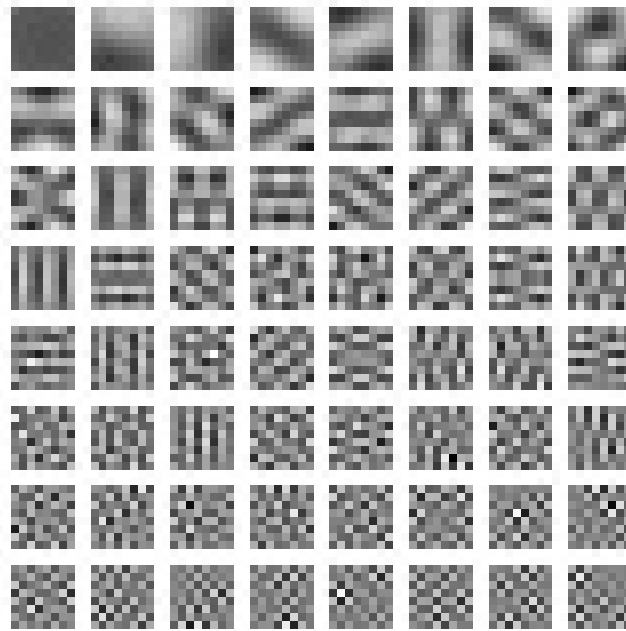
Figure 1. Principal components calculated on 8 \times 8 image patches extracted from natural scenes using Sanger's rule [18]. The functions are not localized, and the vast majority do not at all resemble any known cortical receptive fields. The first few principal components appear 'oriented' only by virtue of the fact that they are composed of a small number of low frequency components (since the lowest spatial frequencies account for the greatest part of the variance in natural scenes [7]), and reconstructions based solely on these functions will merely yield blurry images.
