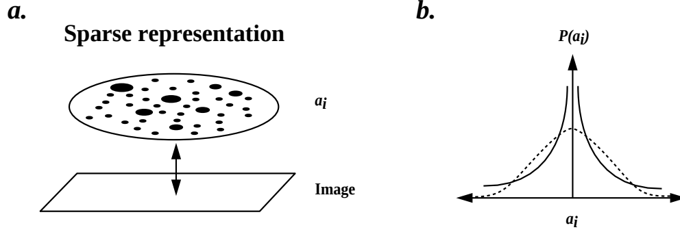
Figure 3. Sparse coding. (a) An image would be represented by a small number of ‘active’ coefficients, a_i , out of a large set. Which coefficients are active varies from one image to the next. (b) The distribution of activity on any given unit should be peaked around zero with heavy tails. Such a distribution will have low entropy, as opposed to a Gaussian distribution (broken line) which has maximum entropy for the same variance.
