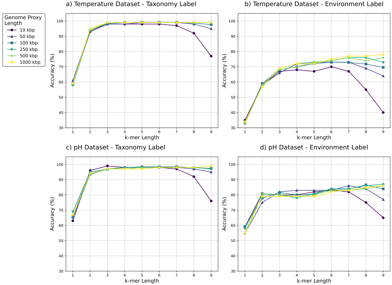
Fig. 3. Classification accuracy of SVM classifier under bias mitigation scenario. a : Temperature Dataset with taxonomy labels. b : Temperature Dataset with environment-type labels. c : pH Dataset with taxonomy labels. d : pH Dataset with environment-type labels. Each subfigure shows accuracy across nine k -mer sizes and six genome proxy lengths.
