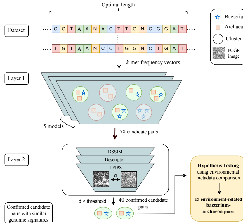
Fig. 4. Multi-layered pipeline for identifying bacterium-archaeon pairs with similar genomic signatures. Layer 1 : Five selected non-parametric clustering methods identify clusters of organisms with similar genomic signatures. The clusters containing both bacteria and archaea (green) generate a list of 78 candidate bacterium-archaeon pairs, grouped by these algorithms based on their similar genomic signatures. Layer 2 : The candidate pairs from Layer 1 undergo pairwise distance calculations between their FCGRs using four different distance metrics. Only 40 pairs, with the majority of distances below empirically determined thresholds, are retained. Hypothesis Testing : after identifying confirmed candidate bacterium-archaeon pairs with similar genomic signatures, a biological analysis is conducted. This includes checking environment labels and examining metadata about their living environments to select pairs isolated from similar types of extreme environments. The final output is a list of 15 environment-related bacterium-archaeon pairs (comprising 16 unique genera and 20 unique species) that have similar genomic signatures and passed the hypothesis testing. These pairs can confidently be proposed as maximally taxonomically divergent microbes (from different domains, Bacteria and Archaea) that share similar genomic signatures associated with their living environments.
