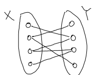
maximum matching
