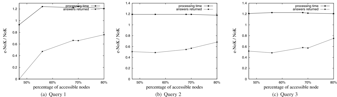
Figure 7. Performance between \epsilon -NoK and NoK as a function of node accessibility
