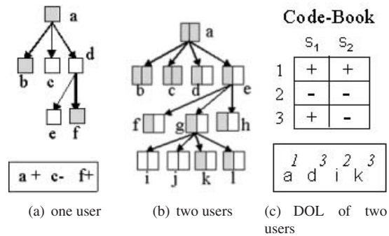
Figure 1. XML data with fine-grained access control and its DOL
