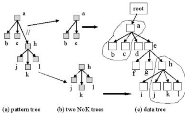
Figure 2. A Pattern Tree with two NoK trees matched to data tree
