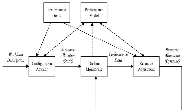
Figure 3: Virtualization design advisor.
