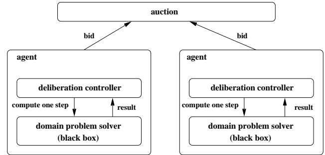
Figure 2: An auction with two computationally restricted agents. In order to submit a reasonable bid, each agent needs to first (approximately) compute its valuations for the item that is up for auction.
