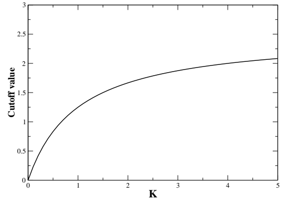
Figure 4: The cutoff values for agent i as a function of K . For each value of K , if agent i 's cost of computation falls below the line then it will compute. Otherwise, it does not. In this example, V = 5 .
