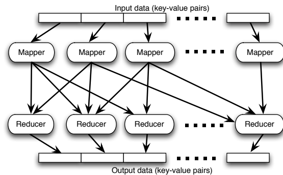
Fig. 1. The architecture of the MapReduce framework
