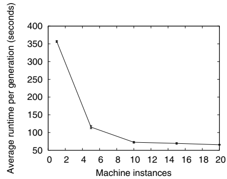
Fig. 4. The effects of cluster size
