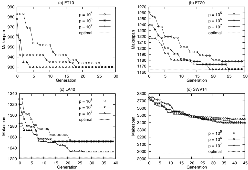
Fig. 3. The results of GA with various population sizes p for the problems (a) FT10, (b) FT20, (c) LA40, and (d) SWV14
