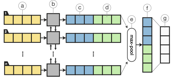
Figure 1: Illustration of the model architecture, where the labels are the following: (a) input word embeddings (b) BiLSTM (c, d) concatenated forward h_{1:n}^f and backward h_{1:n}^b hidden features (e) max-pooling over time (f) document feature vector (g) softmax or sigmoid output.
