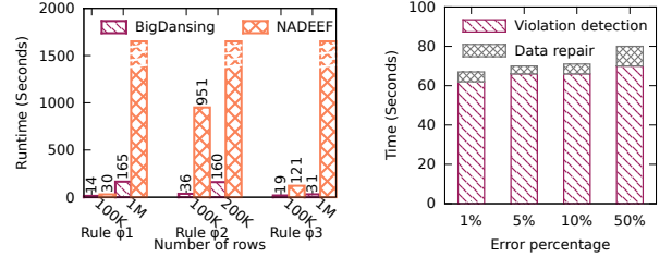
(a) Rules \varphi_1 , \varphi_2 , and \varphi_3 .
