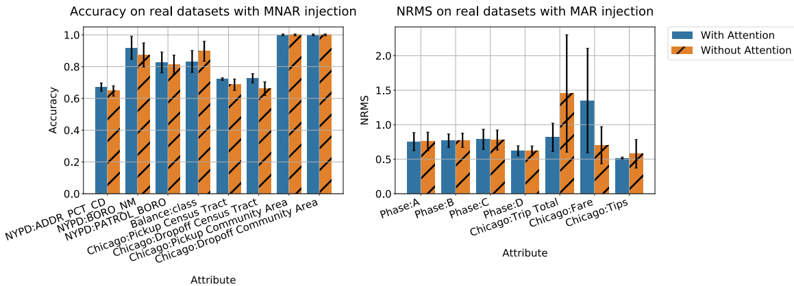
Figure 9: Imputation Accuracy and NRMS error on real data sets under MNAR/MAR injections of AimNet with and without attention layer.
