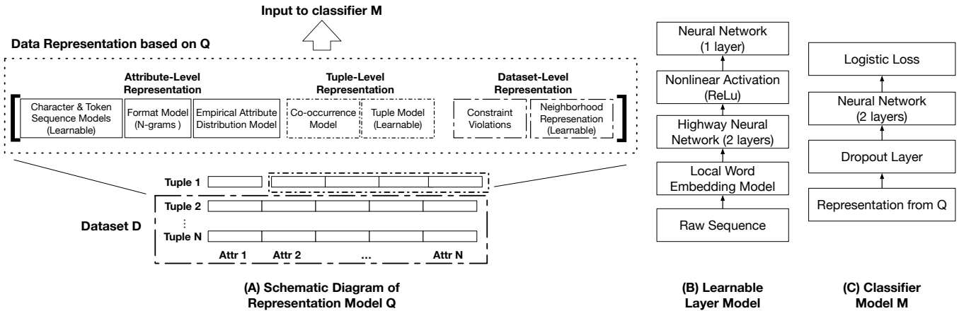
Figure 2: (A) A diagram of the representation model Q. Models associated learnable layers that are jointly trained with classifier M. (B) Architecture diagram of the learnable layers in Q. (C) The architecture of classifier M.
