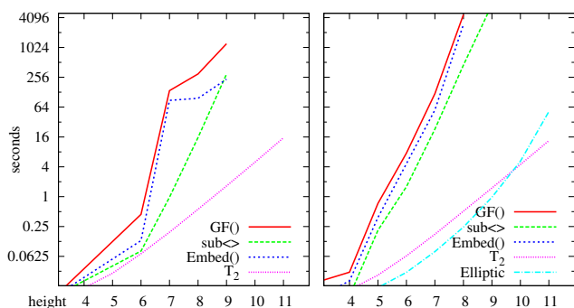
Figure 3: Times for building 3-adic towers on top of \mathbb{F}_2 (left) and \mathbb{F}_5 (right), in Magma (first three lines) and using our code.
