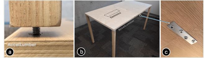
Figure 7: Fabrication of a desk using AccelLumber panels. (a) Attach the legs by screwing them into pre-drilled pilot holes within an AccelLumber panel. (b) The completed desk assembly. The dashed box indicates the location of the electronic components (power management, BLE, MCU, and accelerometer) embedded within the panel. (c) The desktop was constructed using two AccelLumber panels joined with flat brace brackets.
