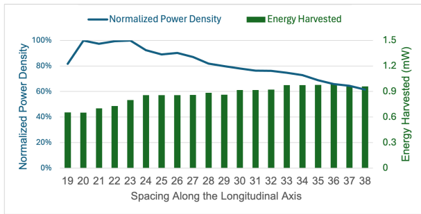
Figure 13: The effect of longitudinal spacing on the energy harvested by the central antenna (green bars, y-axis on the right), and power density (blue line, y-axis on the left) for the 3-antenna array.
