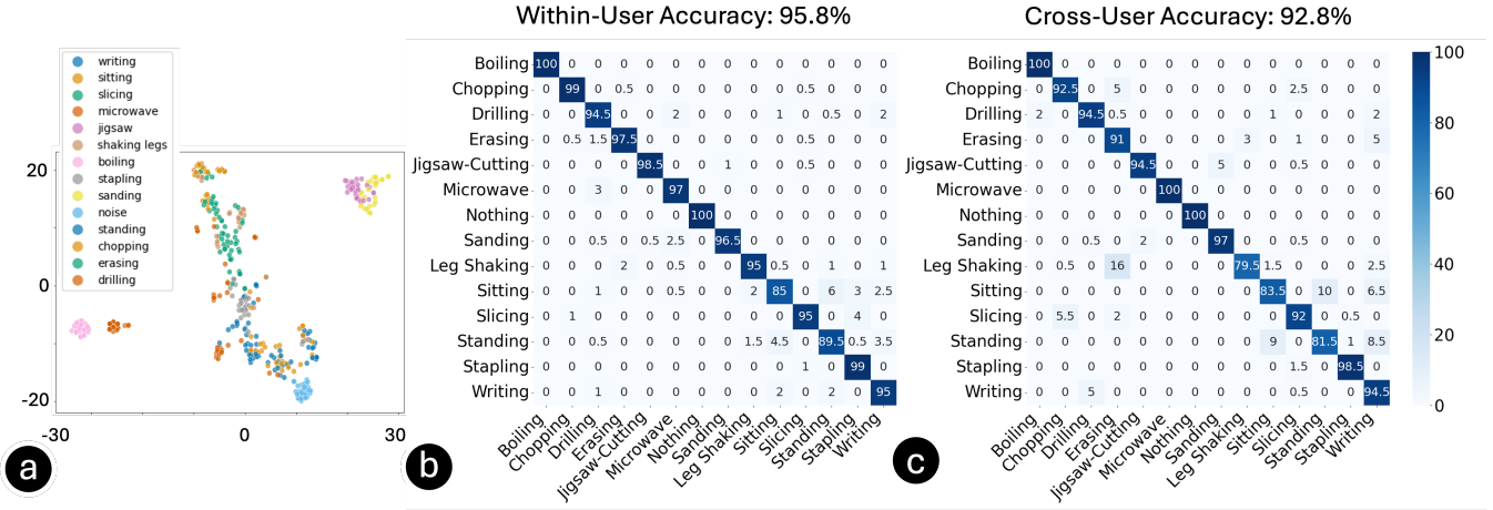
Figure 11: (a) t-SNE plot of the activity data. (b) Confusion matrix showing classification accuracy in the within-user scenario. (c) Confusion matrix showing classification accuracy in the cross-user scenario. All results are based on a model trained using data collected from the desk and stool.
