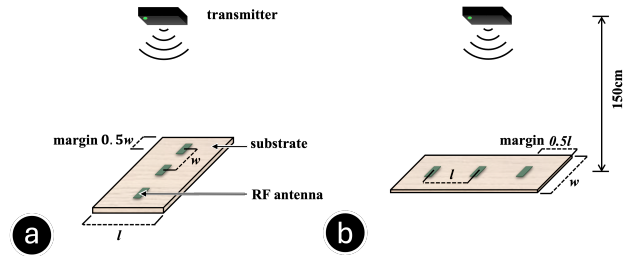
Figure 12: The experiment setup for (a) a 3 \times 1 antenna array and (b) a 1 \times 3 antenna array.
