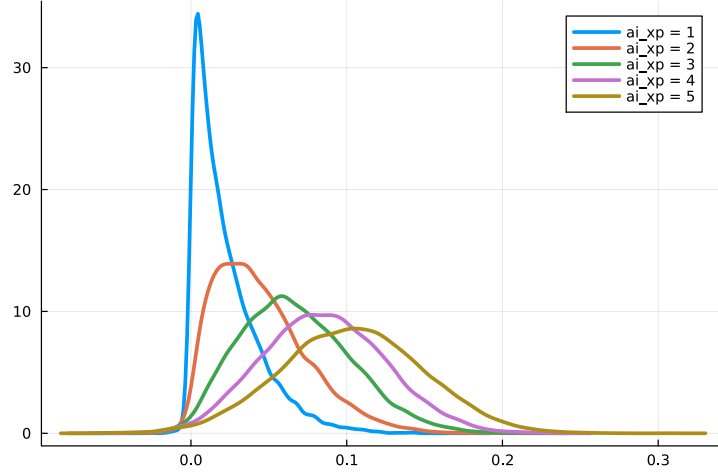
Fig. 21: Posterior effect of AI use in Task 1 on CH after manual evolution in Task 2. The effect is negligible when Task 1 developers had minimal AI skills but increases with more habitual use.
