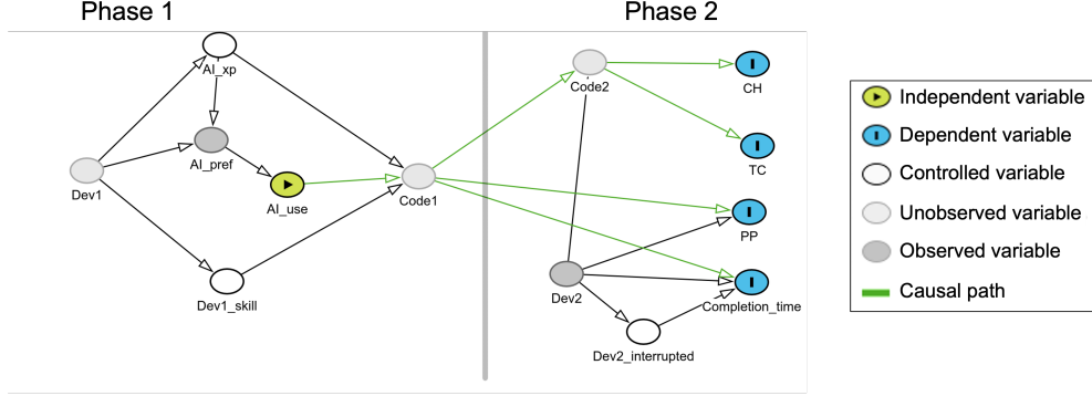
Fig. 5: DAGitty causal graph. Dev1 and Dev2 represent the full complexity of the human participants in Phases 1 and 2, respectively. Code1 and Code2 are the participants’ solutions after Phases 1 and 2, respectively. AI_use is the independent variable. The other variables are explained in Table 3.
