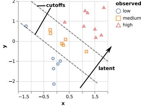
Fig. 6: A diagram explaining an ordered logistic regression model. If we observe the two predictors x and y , as well as the observed responses ( observed ). The model infers both a latent score ( latent ) for each point (as a linear combination of x and y ), and cutoffs between the different response levels. In other words, the model finds hyperplanes separating each response level with the next, where all hyperplanes are parallel.
