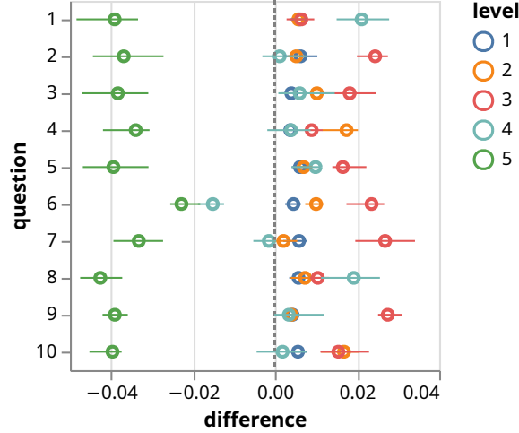
Fig. 19: Difference in predicted responses for a habitual AI user with an advanced level of Java, comparing evolution of AI-assisted vs. non-assisted solutions. Each row represents a survey question and the x-axis shows changes in response probabilities. Developers evolving AI-assisted code are about 4 percentage points less likely to answer 5 (“fully agree”) and slightly more likely to answer 3 (“neutral”). The overall effect is small but consistent.
