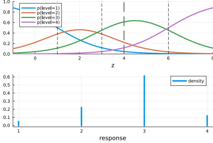
Fig. 23: Two plots, showing the relationship between the latent variable z and an ordered logistic distribution with cutoffs [1, 3, 6] . The top plot shows the probability of each of the 4 levels as a function of z , where the cutoffs are shown using black dashed lines. The bottom plot shows the probability of each response level for z = 4 . The bottom plot is a slice indicated on the top plot by a gray dashed line. As z increases, higher response levels become more probable, but there is no assumption that cutoff levels are evenly separated.
