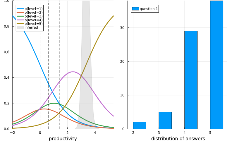
Fig. 18: Relationship between inferred productivity and responses to question 1. The left-hand plot shows the probability of each response level being observed based on the productivity on the x-axis. The shaded area shows an inferred productivity approximately between 3-4 points. The dashed lines indicate the inferred cutoffs between response levels. Looking at the curves, we can see that for a productivity in that range, the most likely answers for question 1 are level 5 (highest curve) or 4, and perhaps a few 3. This is consistent with the observed responses, showed on the right-hand plot.
