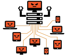
Botnet Detection
