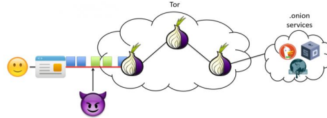
Website Fingerprinting
