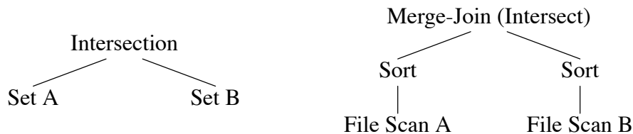
Figure 3. Logical and Physical Algebra Expressions.
