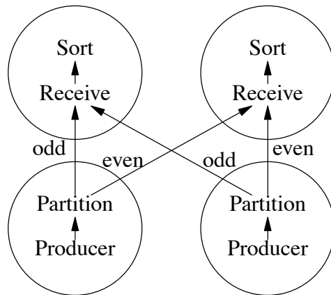
Figure 38. Deadlock-Free Scenario.
