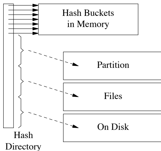
Figure 9. Hybrid Hashing.
