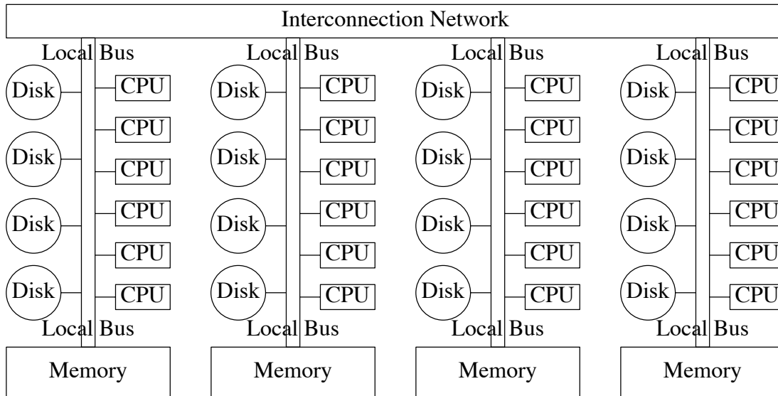
Figure 36. A Hierarchical-Memory Architecture.
