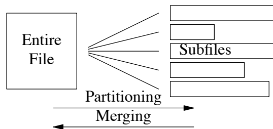
Figure 23. Partitioning Skew.
