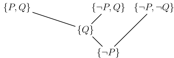
Figure 2: Resolution DAG D' = \text{percolate}(D, A, L)
