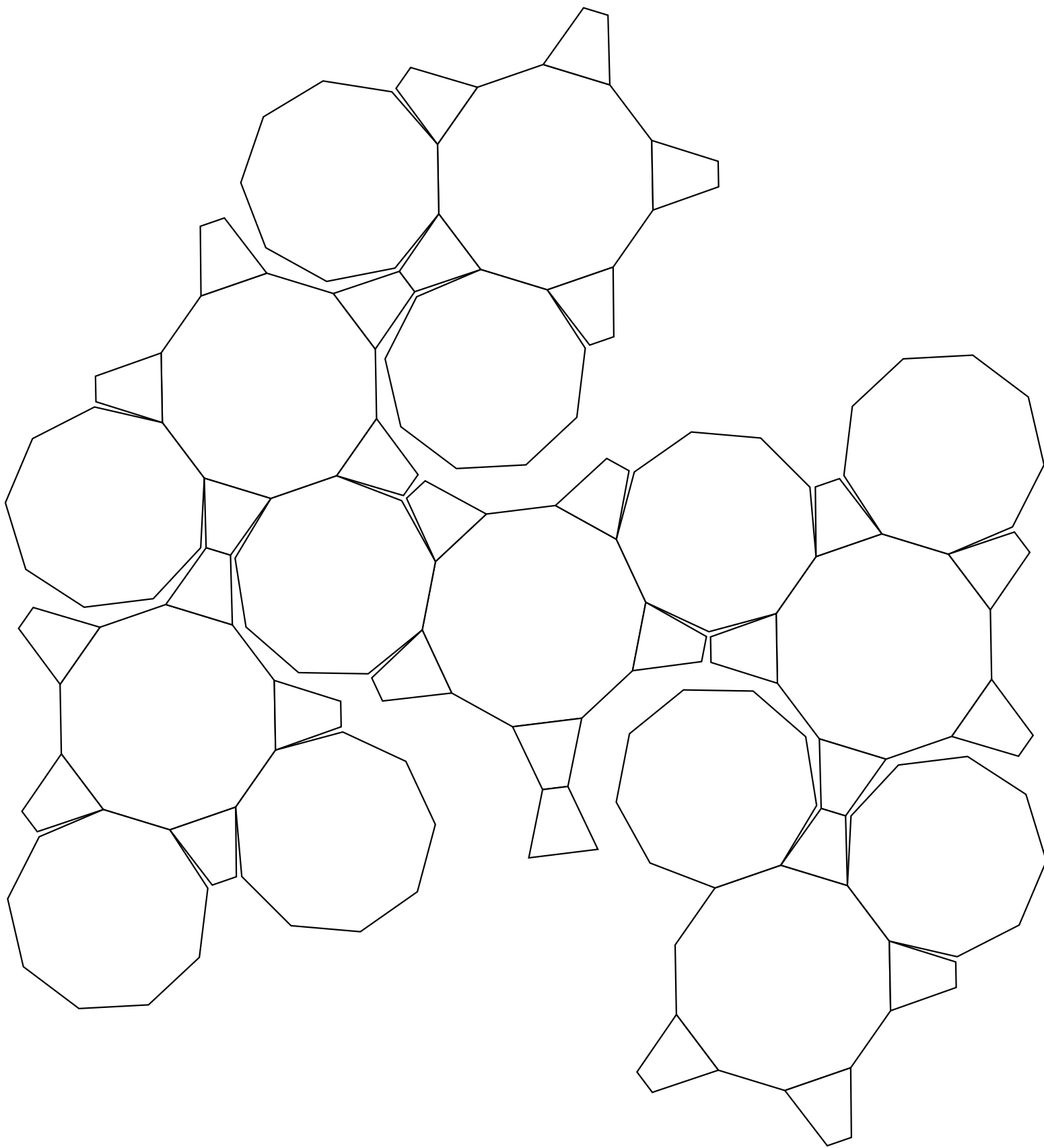
Folding net for one half of the "bowtie icosahedron" I(2,3,*,e)
