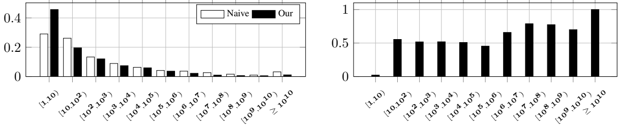
(a) Distribution of the numbers of variants. For example, the first pair of vertical bars shows that 29% of the test programs have fewer than 10 variants enumerated using the naïve approach. The percentage increases to 46% using our approach.
