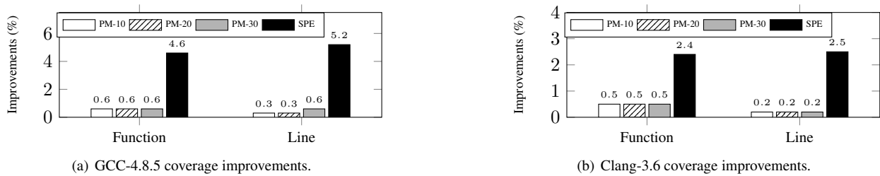
Figure 9. Coverage improvements over the baseline tests. PM-X represent improvements achieved by program mutation (the Orion tool) which deletes X statements, and SPE represents improvements achieved using our SPE algorithm.
