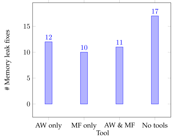
Fig. 3. Distribution of memory leak fixes by AddressWatcher (AW) and Memfix (MF).
