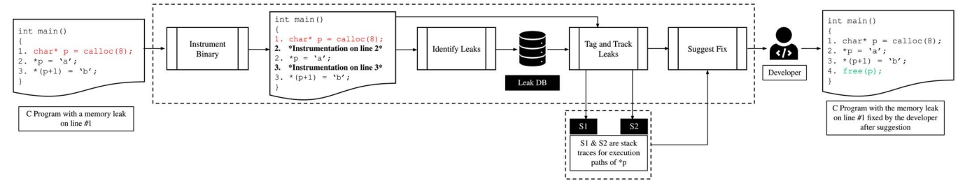
Fig. 2. An overview of our approach for suggesting a location of a memory leak fix.
