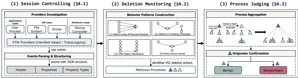
Fig. 1. Overall workflow of REMEMBRALL. It contains three modules: Session Controlling, Deletion Monitoring, and Process Judging. If ransomware is detected, all corresponding processes will be killed, and the system backup disruption attack (i.e., VSCs deletion) will be terminated.
