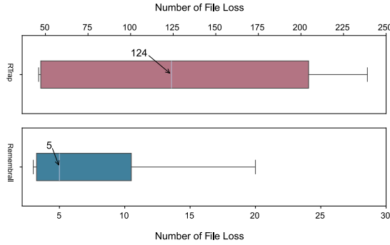
Fig. 3. The number of files that have been encrypted when the anti-ransomware tool detects attacks. Given that ransomware’s goal is to encrypt as many files as possible, the file loss metric reflects the detection latency of real-time security tools.
