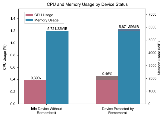
Fig. 4. CPU and memory usage of REMEMBRALL on a freshly booted machine. The first ‘Idle Device’ group shows hardware usage without REMEMBRALL installed, while the increments in the second group reflect REMEMBRALL’s overhead - 0.07% CPU and 150.27 MiB memory.
