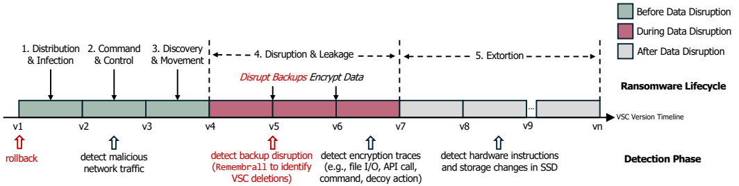
Fig. 5. Ransomware lifecycle stages and corresponding mitigation efforts. Our work targets an unexplored phase - detecting backup disruption - where current approaches fall short, distinct from previous research on network traffic, encryption traces, SSD logs, etc.
