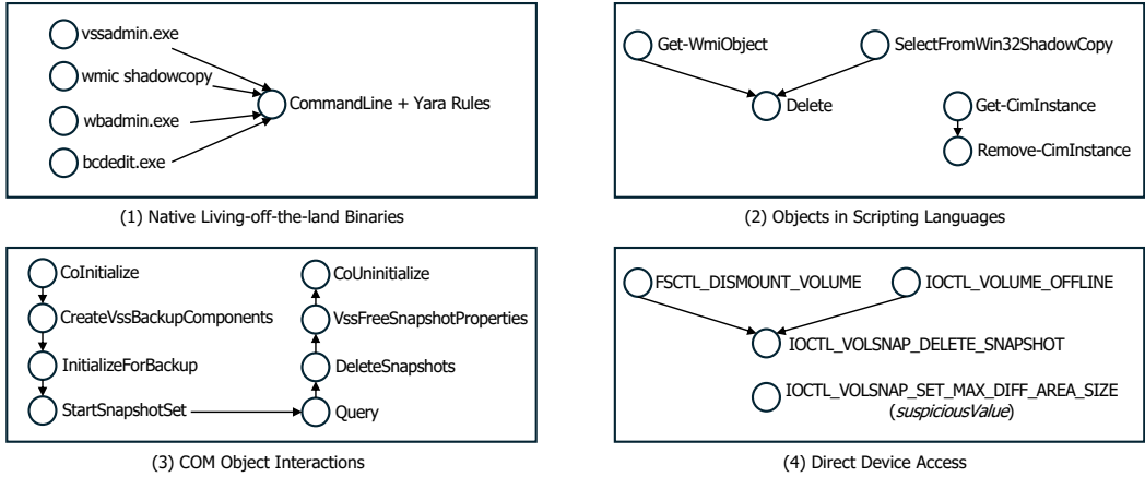
Fig. 2. The high-level behavior patterns for four types of system backup disruptions that we proposed in Section 3. We follow these patterns to monitor the VSC deletion attacks from native living-off-the-land binaries, objects in scripting languages, COM object interactions, and direct device access, respectively.
