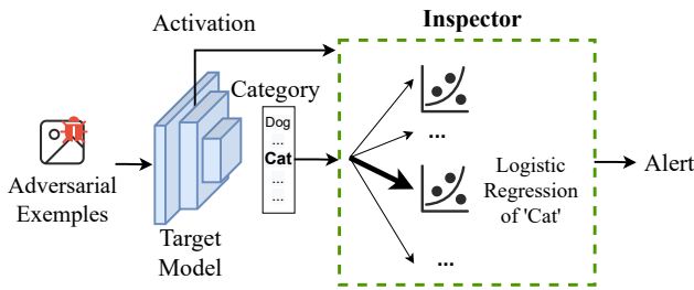
Figure 4: Structure of Inspector . It leverages per-category logistic regression models to catch adversarial examples.
