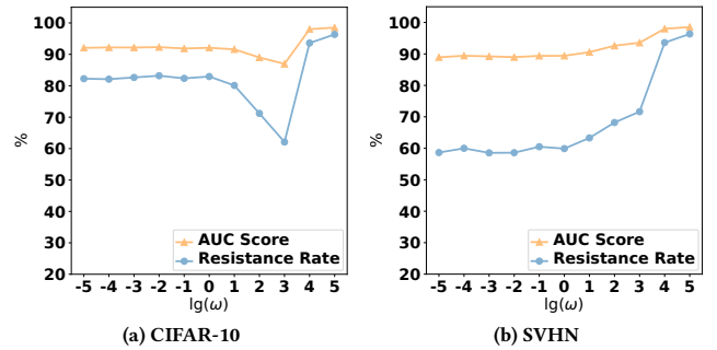
Figure 6: Resistance rate and AUC score of COOPHANCE under adaptive attack. Figure 6a and Figure 6b are evaluated on CIFAR-10 and SVHN, respectively.
