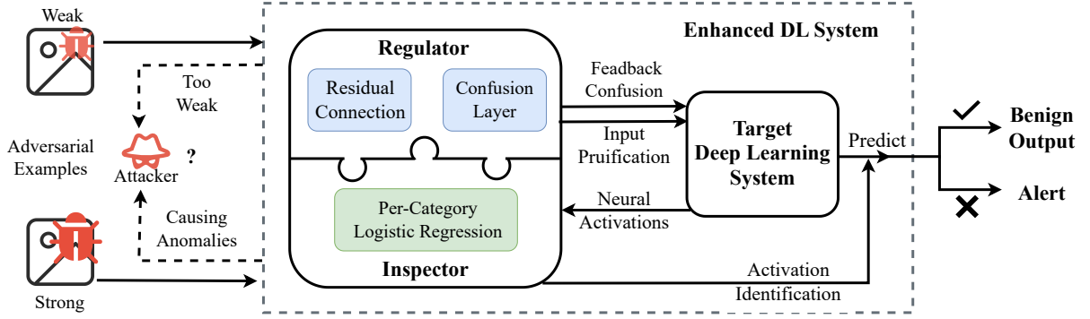
Figure 2: Overview of COOPHANCE. Regulator regulates the input image to purify adversarial examples and confuses the feedback gradient to hinder adversarial example generation. Inspector can identify whether the input image is malicious based on the neuron activations of the target system. With them, COOPHANCE can either help the target system give the benign output or alert developers to potential attacks., leaving attackers two attack objectives in contradictory directions.
