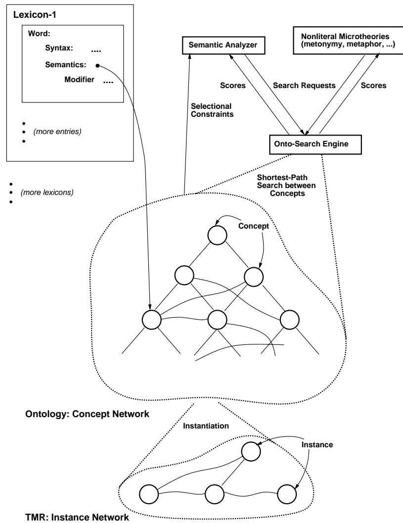
Figure 1: The Role of the Ontology in Mikrokosmos
