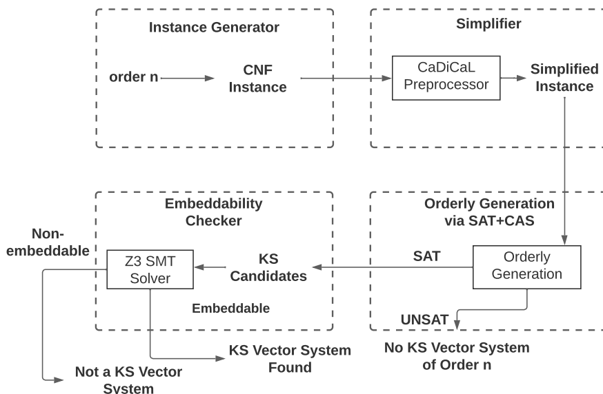
Fig. 1: A flowchart of our SAT+CAS based tool PhysicsCheck for solving the KS problem. The instance generator generates the SAT instance encoding the KS problem (see Section 4), and the instance is simplified using CaDiCaL [29]. The simplified instance is passed to the MapleSAT+CAS tool (see Section 5) either sequentially or in parallel using cube-and-conquer [30]. Finally, an embeddability checker applies the SMT solver Z3 to determine whether the candidates are embeddable (see Section 6).
