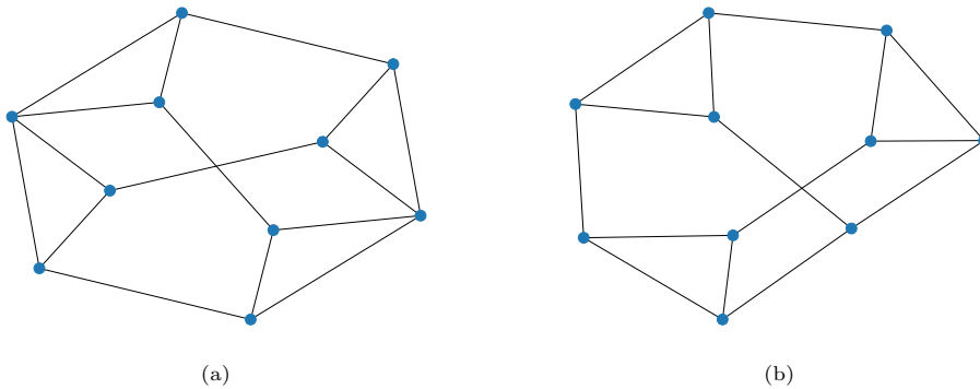
Fig. 4: The only two minimal nonembeddable graphs of order 10. These are the smallest squarefree graphs that are not embeddable.
