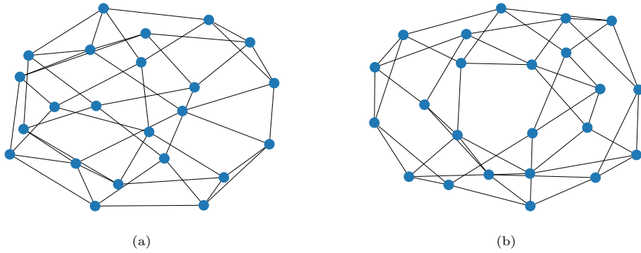
Fig. 6: The only two KS candidates up to order 23 that do not contain minimal nonembeddable graphs up to and including order 14. These two graphs are determined to be unembeddable by Z3.
