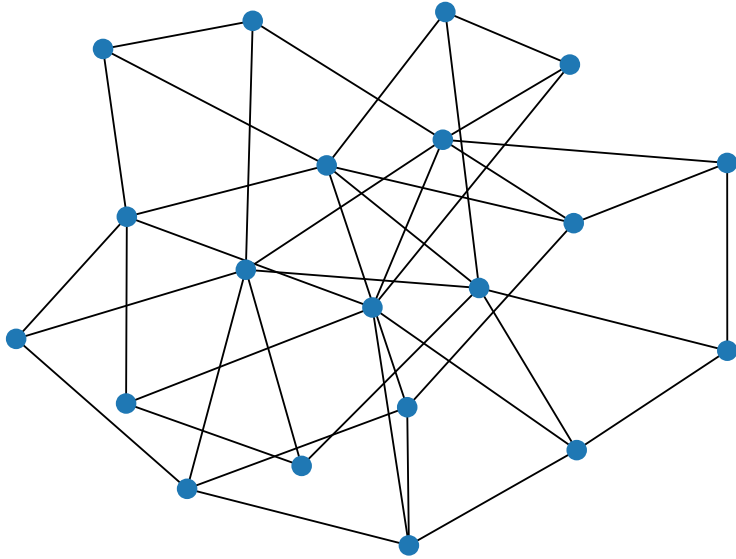
Fig. 5: One of the four graphs with 20 vertices that was not present in Uijlen and Westerbaan’s enumeration. The four graphs satisfy all constraints mentioned in Section 4, but are not embeddable, and therefore do not constitute a KS system.
