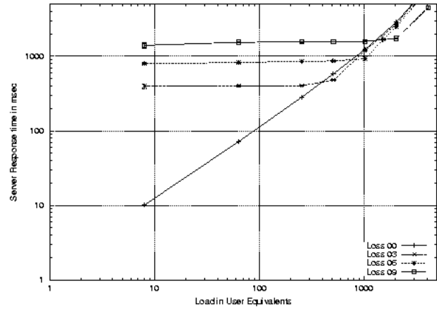
Figure 13: Flash Response Time vs. Dependent Loss Rate
