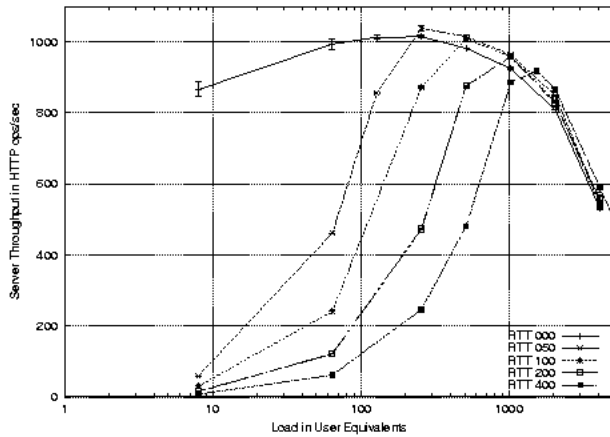
Figure 11: Flash Throughput vs. RTT
