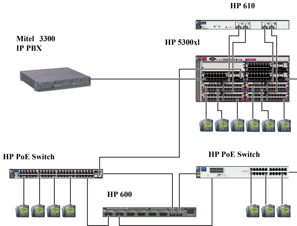
Figure 1-1. Example of a Typical Implementation
