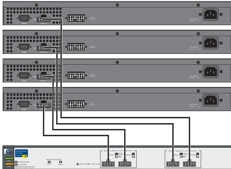
Figure 3-5. Example of an HP 610 EPS Powering Four Switches
