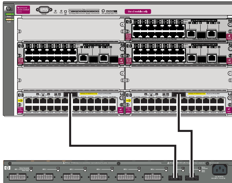
Figure 3-7. Example of an HP 600 RPS/EPS Powering Two Modules
