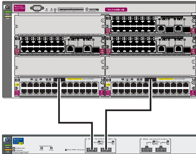
Figure 3-9. Example of an HP 610 EPS Powering Two Modules
