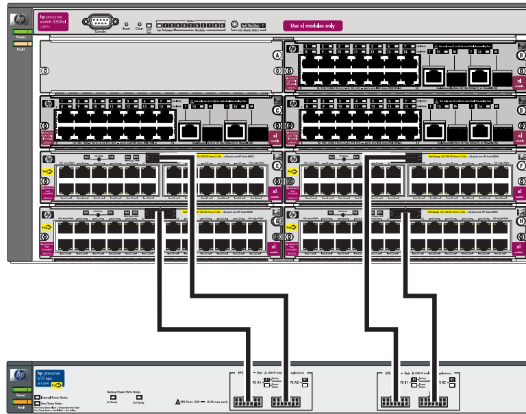
Figure 3-10. Example of an HP 610 EPS Powering Four Modules
