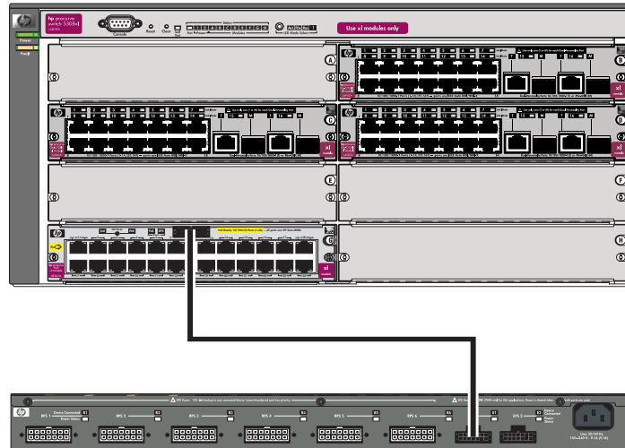
Figure 3-6. Example of an HP 600 RPS/EPS Powering One Module
