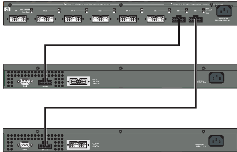
Figure 3-4. Example of an HP 600 RPS/EPS Powering Two Switches
