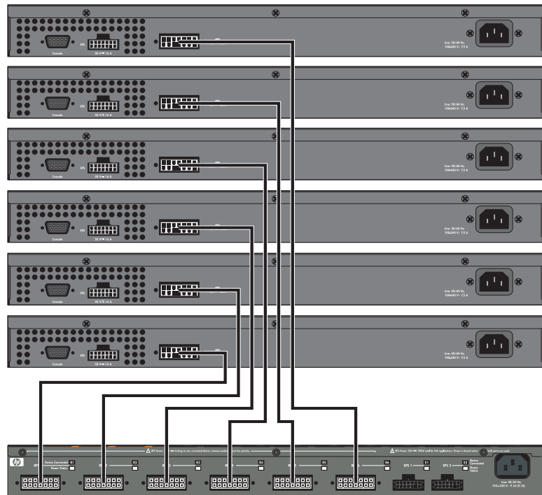
Figure 2-1. Example RPS Connections on the HP 600 RPS/EPS
