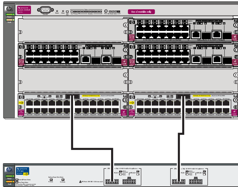
Figure 3-8. Example of an HP 610 EPS Powering Two Modules
