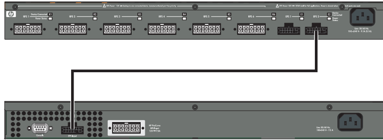
Figure 3-3. Example of an HP 600 RPS/EPS Power One Switch
