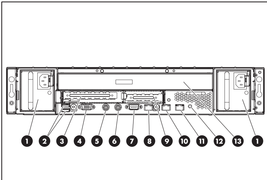
Figure 32 DL320s rear panel
