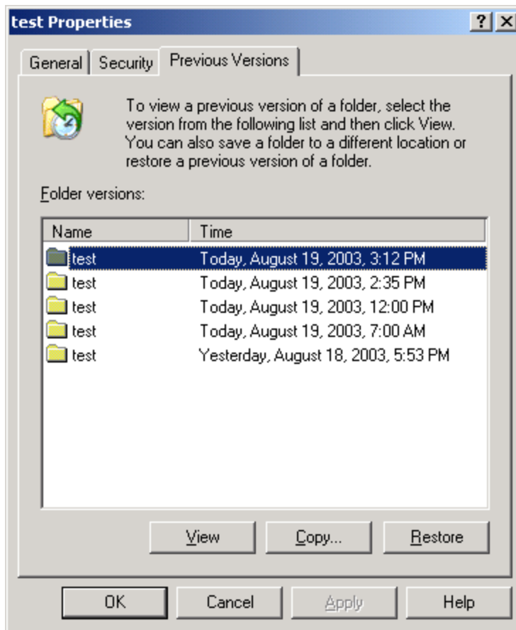
Figure 12 Recovering a deleted file or folder
