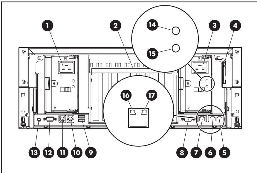
Figure 36 DL585 G2 rear panel
