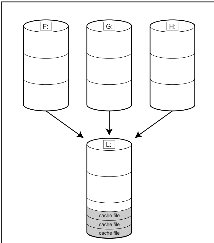
Figure 9 Shadow copies stored on a separate volume
