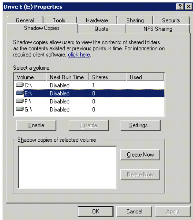
Figure 10 Accessing shadow copies from My Computer
