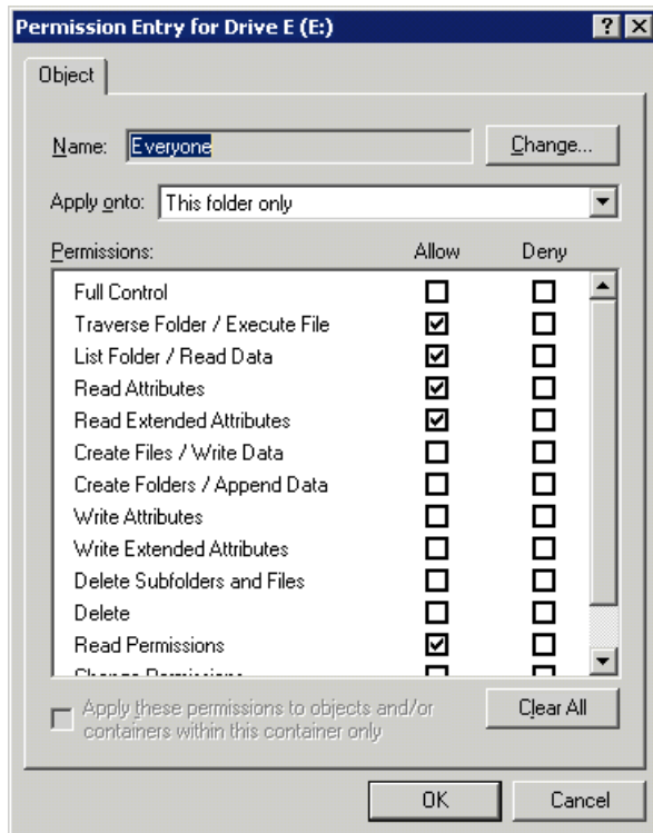
Figure 15 User or group Permission Entry dialog box
