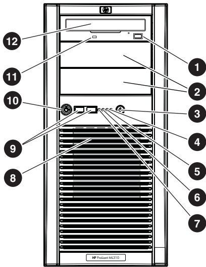
Figure 29 ML310 G4 front panel
