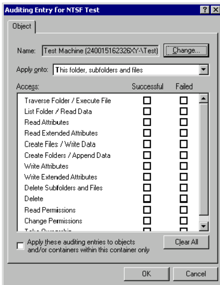
Figure 18 Auditing Entry dialog box for folder name NTFS Test
