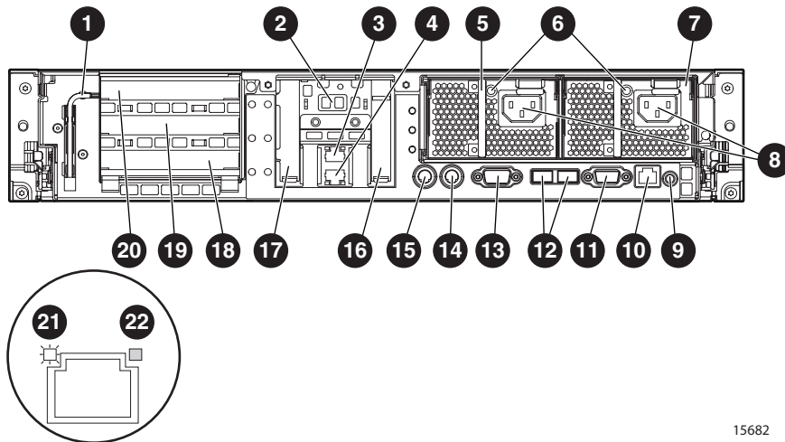
Figure 34 DL380 G5 rear panel
