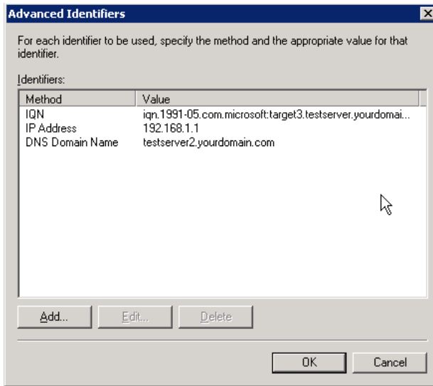
Figure 25 Advanced Identifiers page
