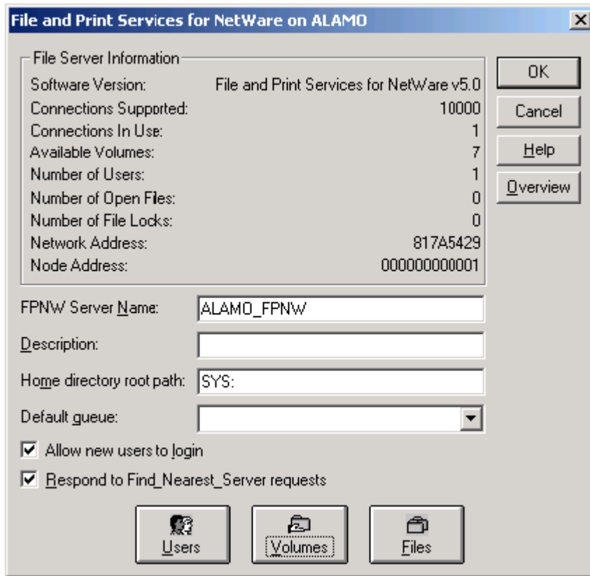
Figure 21 File and Print Services for NetWare dialog box
