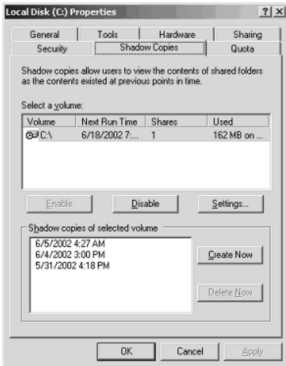
Figure 7 System administrator view of Shadow Copies for Shared Folders
