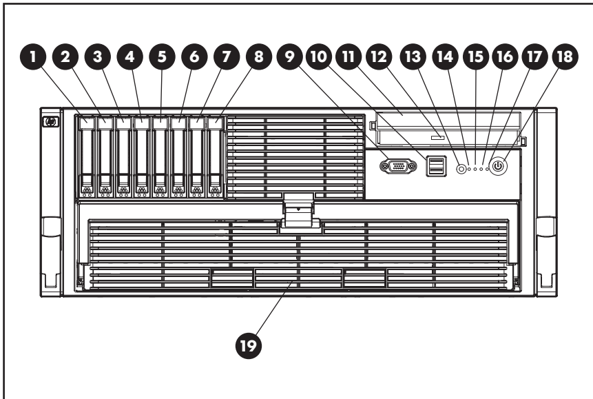
Figure 35 DL585 G2 front panel
