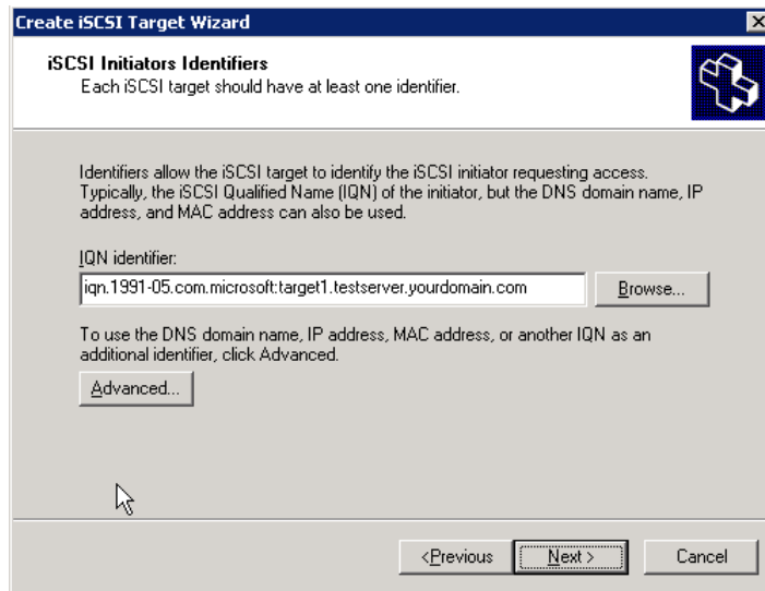
Figure 24 iSCSI Initiators Identifiers page
