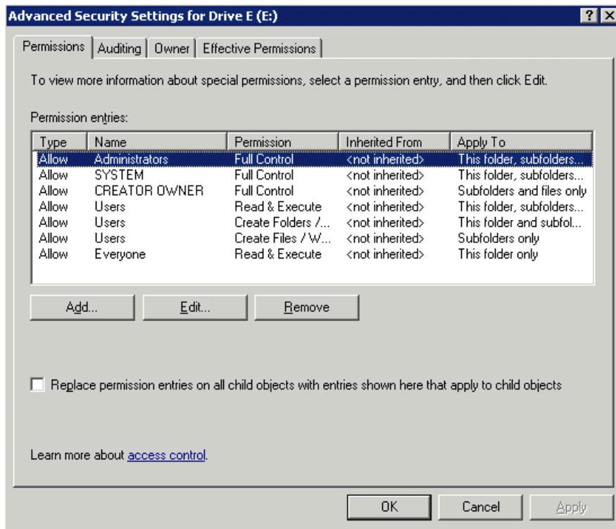
Figure 14 Advanced Security settings dialog box, Permissions tab
